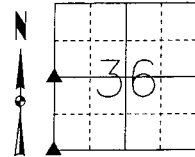
WEST 1/4 CORNER FOUND CONCRETE MONUMENT & SET 1/2" REBAR CAP #11804
