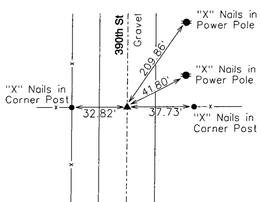
WEST 1/4 CORNER FOUND CONCRETE MONUMENT & SET 1/2" REBAR CAP #11804
