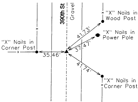
SOUTHWEST CORNER FOUND CONCRETE MONUMENT & SET 1/2" REBAR CAP #11804
