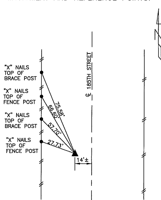
DISTANCES PLUMB CHAINED CENTER OF SECTION 16-82-40
