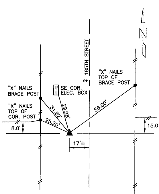
DISTANCES PLUMB CHAINED SW CORNER NW1/4 NE1/4 SECTION 16-82-40
