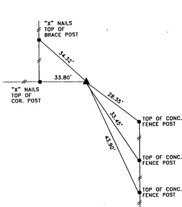
DISTANCES SLOPE CHAINED W1/4 CORNER SECTION 4-85-38
