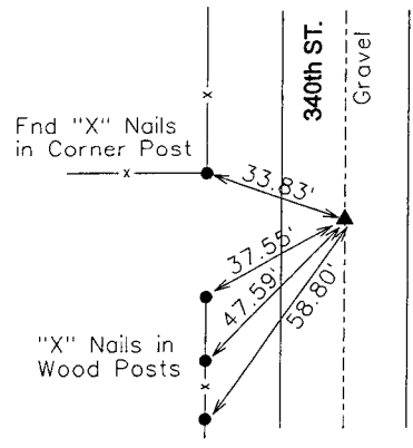
E 1/4 CORNER FOUND CONCRETE MONUMENT
