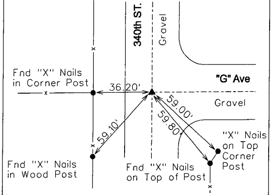
SOUTHEAST CORNER FOUND 1/2" BOLT
