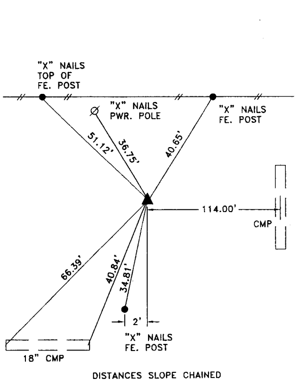
S1/4 CORNER SECTION 26-84-40
