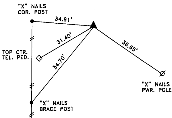
DISTANCES SLOPE CHAINED SW CORNER SE1/4 SW1/4 SECTION 7-83-38
