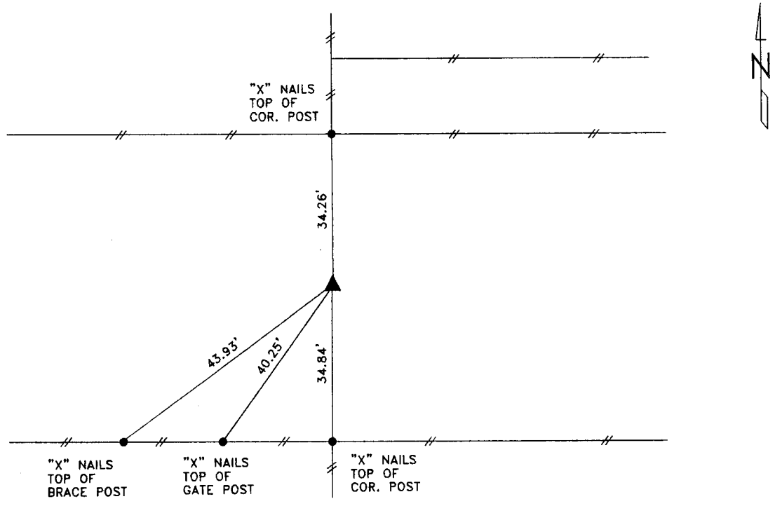
DISTANCES SLOPE CHAINED N1/4 CORNER SECTION 24-84-41
